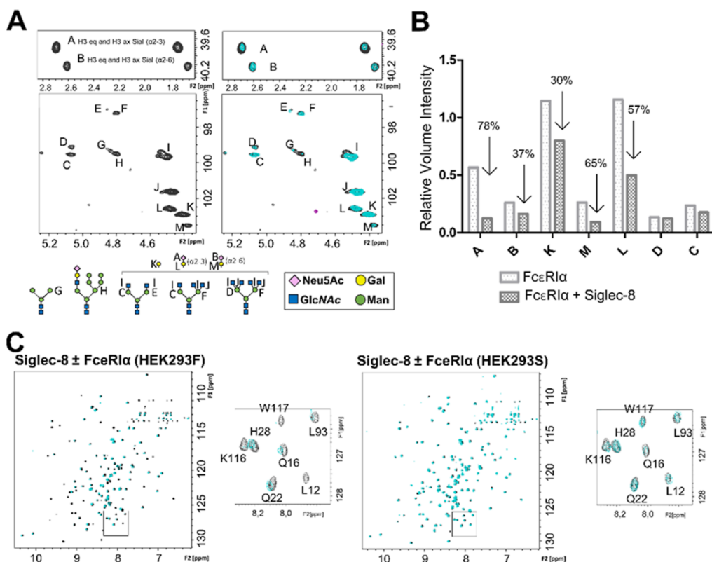
Figure 5. Interaction of the ECD of Siglec-8 with the sialylated N-linked glycans of Fc \epsilon R1 \alpha as measured by NMR. (A) Expansion of the anomeric region and the region containing the axial and equatorial H3 protons of the Neu5Ac residues of Fc \epsilon R1 \alpha expressed in HEK293F cells. On the right-hand side, the glycan composition of Fc \epsilon R1 \alpha under physiological conditions is represented (black), and on the left-hand side, the superimposition of glycan spectra in the absence (black) and presence of 5 equiv of Siglec-8 d1 (cyan). Note the selective loss of intensity for the NMR signals of sialic acid. The glycan composition of Fc \epsilon R1 \alpha was deduced by direct analysis of the [ ^1\text{H} , ^{13}\text{C} ]-HSQC NMR spectra. Each carbohydrate is identified by a letter. The different N-glycans present on the glycoprotein expressed in HEK293F cells are represented with Symbol Nomenclature for Glycans [SNFG] symbols. (B) Bar graph representing intensities corresponding to the signals of sialic acid, with and without Siglec-8. All signals were normalized with respect to trimethylsilylpropanoic acid (TSP). (C) Superimposition of ^1\text{H} , ^{15}\text{N} -TROSY experiment of Siglec-8 d1 in the apo form (black) and after the addition of 1 equiv of Fc \epsilon R1 \alpha (green) expressed in HEK293F cells (left) and in HEK293S cells (green) (right).
