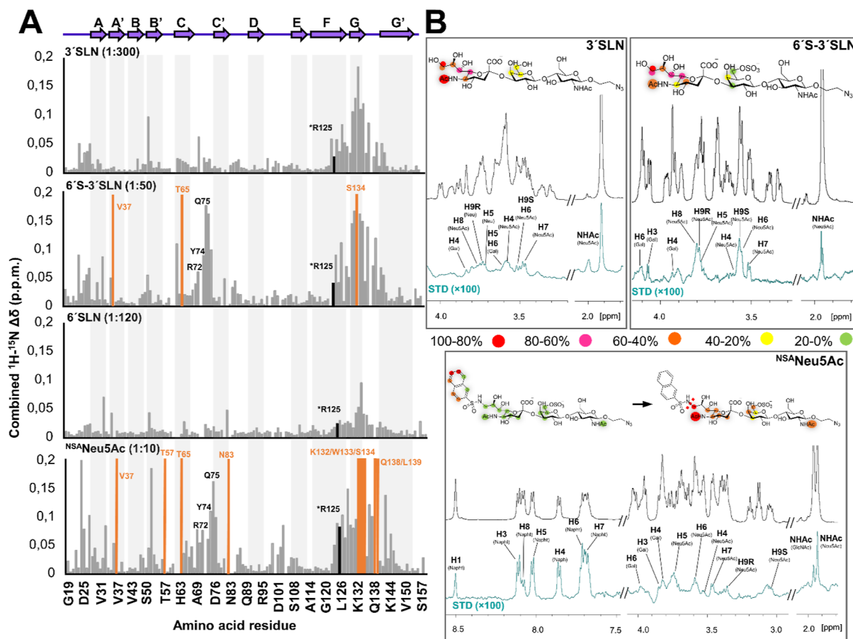
Figure 3. Binding of 3'SLN, 6'-3'SLN, and ^{NSA} Neu5Ac to Siglec-8 measured by NMR spectroscopy. (A) Combined ^1\text{H}-^{15}\text{N} CSPs ( \Delta\delta ) of the ^{15}\text{N} -labeled Siglec-8 d1 residues observed upon titration with the different ligands and at different molar ratios, plotted vs amino acid residues. Secondary structure elements derived from the herein determined crystal structure of Siglec-8 d1 are represented at the top. The residues that experience dramatic signal line broadening during the titration are represented with the orange bars. Residues involved in the interaction with the ligands are also depicted. (B) ^1\text{H} STD-NMR experiments for the complex formed by 3'SLN, 6'-3'SLN and 1:50 for ^{NSA} Neu5Ac. Top: the reference spectrum (black, off-resonance). Bottom: the STD-NMR spectrum (blue) on-resonance was set at the aliphatic region). The ^1\text{H} NMR signals showing the STD effect are annotated. The epitope mapping (relative STD) is shown in the ligand structure. In the case of ^{NSA} Neu5Ac, the epitope mapping was normalized in percentage of the largest signal H6 Napht (left), while the NSA group was not considered, and the epitope was normalized in percentage of the H9S Neu5Ac signal (right).
